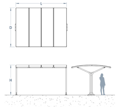
Eastbrook Senior L: 5000mm x D: 3200mm x H: 2305mm
