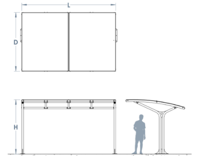
Eastbrook Junior L: 4140mm x D: 2590mm x H: 2305mm (1970mm H to rear)
